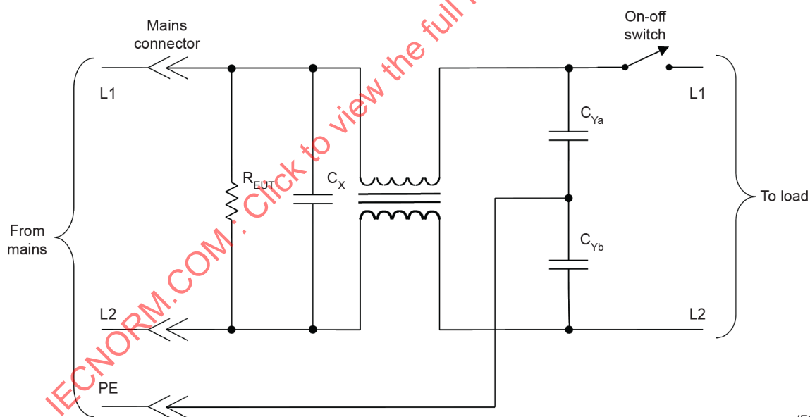
Figure B.1 – Typical EMC filter schematic
