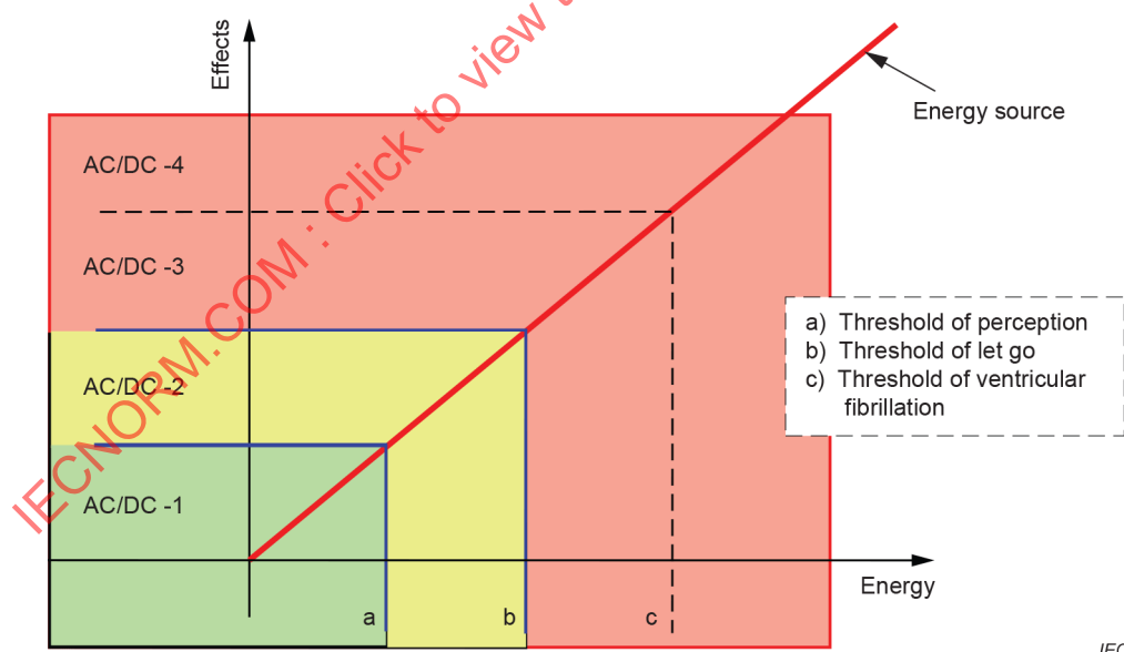
Figure 10 – Illustration that limits depend on both voltage and current
