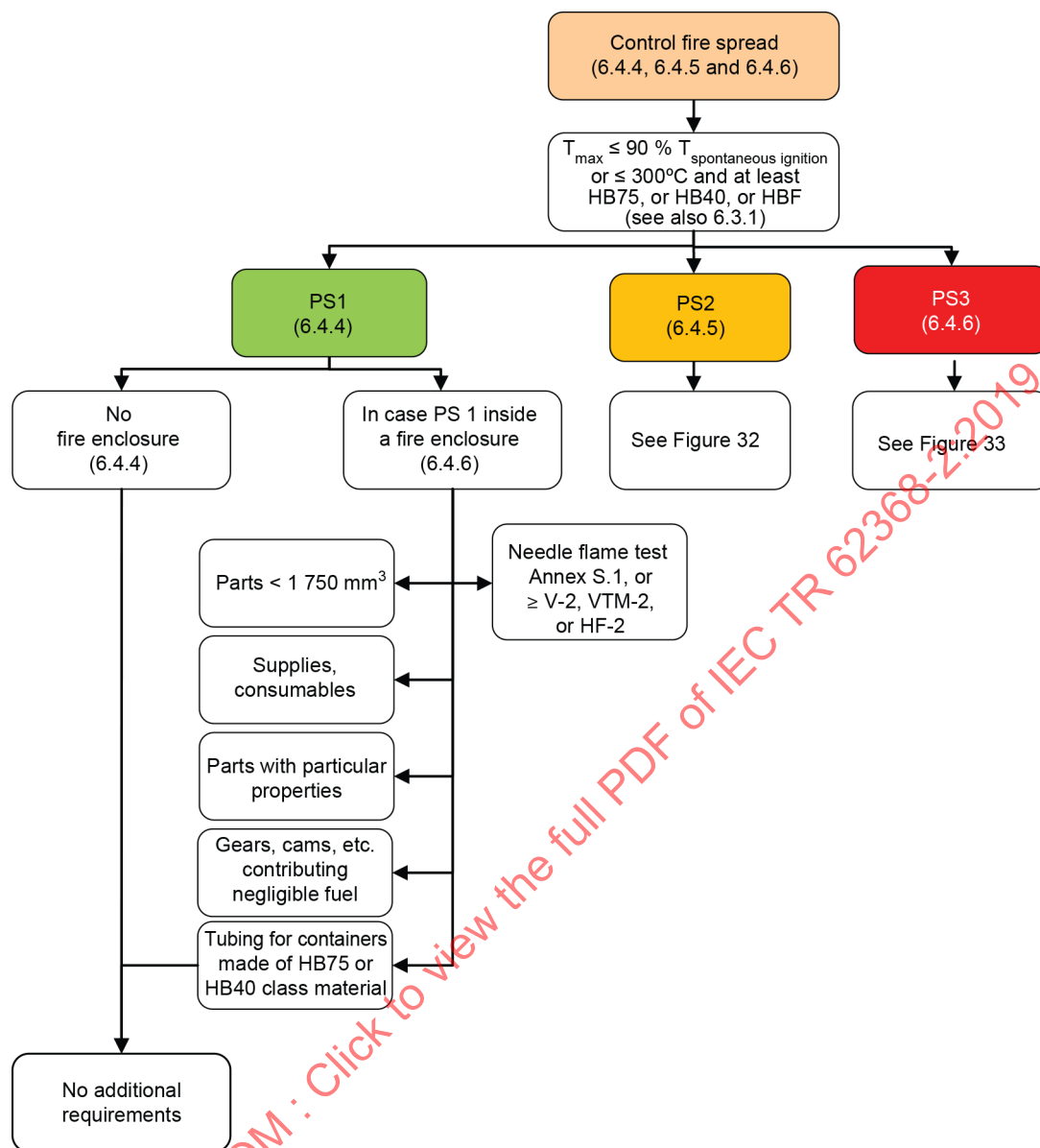
Figure 31 – Control fire spread summary
