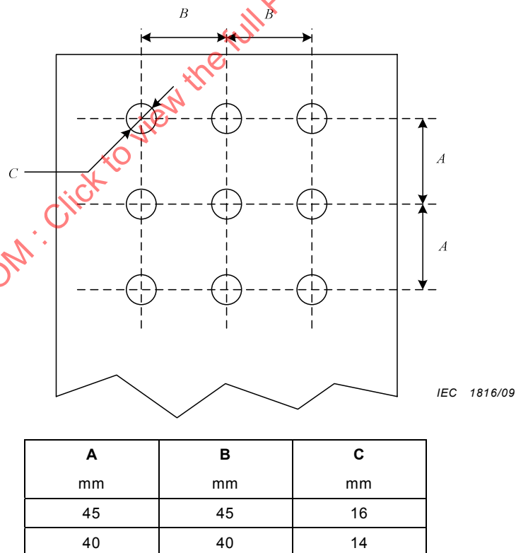
Figure 7 – Nine hole HV terminal (3 × 3 hole pattern)
