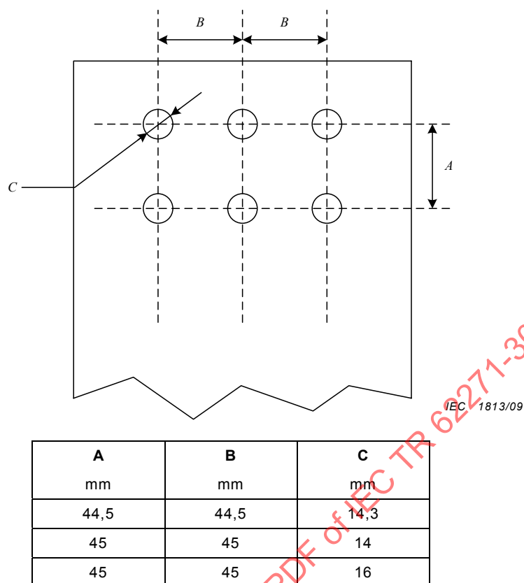
Figure 4 – Six hole HV terminal (2 × 3 hole pattern)
