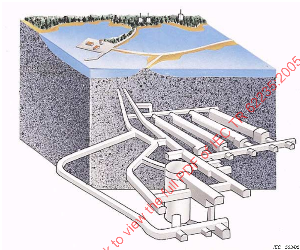
Figure 5 – Layout for the final repository for radioactive operational waste (SFR)
