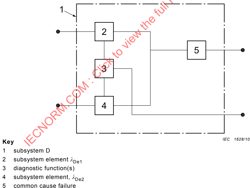
Figure 4 – Logical representation of subsystem D
