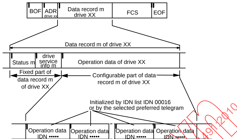
Figure 37 – Structure of the drive telegram
