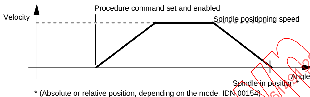
Figure 77 – Velocity diagram for spindle positioning (velocity feedback = 0)
