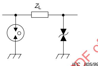
Figure 4 – Circuit de protection type
