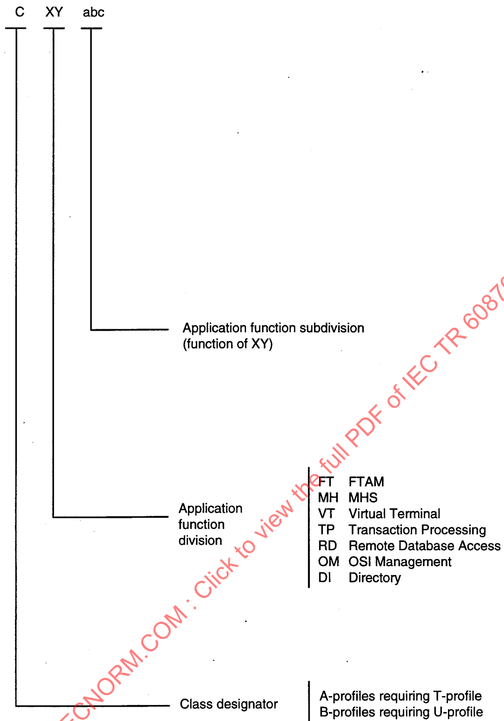
Figure B.2 – Structure of application profile identifier
