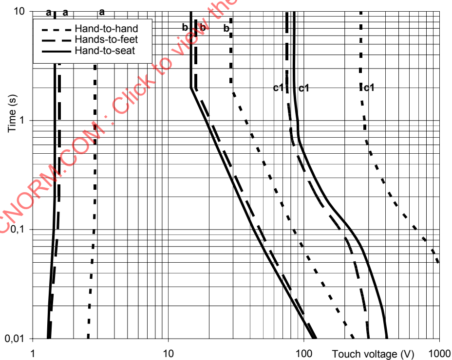
Figure 17 – Conventional time/voltage zones of effects of d.c. current on a person for water-wet condition and large contact area
