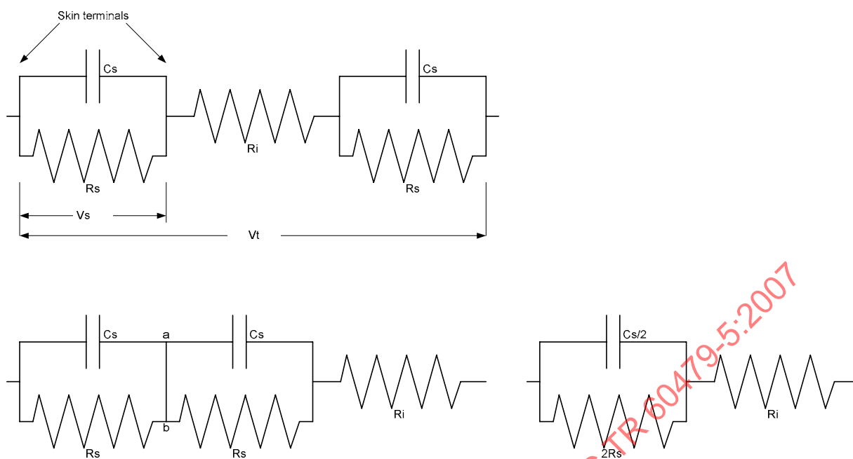
Figure A.1 – Model for hand-to-hand contact
