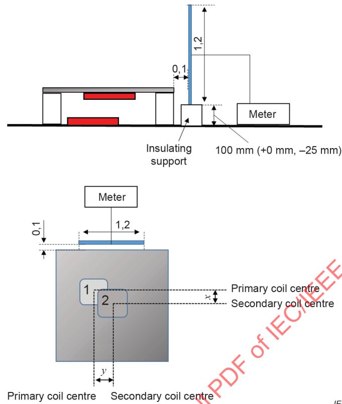
Figure I.12 – Configuration example of contact current with ungrounded condition: (2) with vehicle mimic plate
