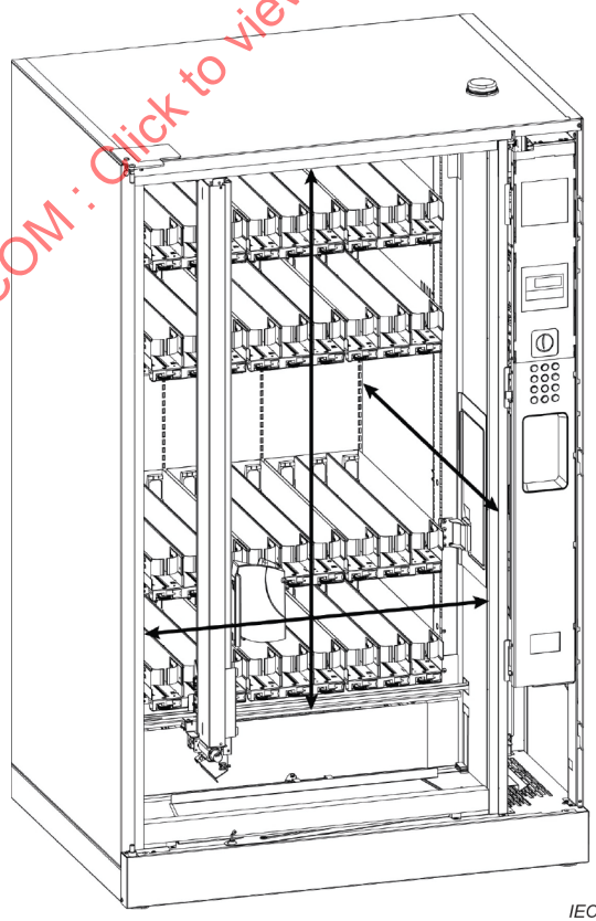
Figure B.3 – Glass fronted can/bottle machine
