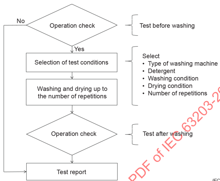
Figure 1 – Flow chart of test procedure
