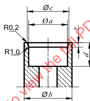
Figure 6 – Gauge for plug outer contact
