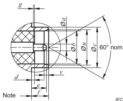
a) RF channel with pin contact
