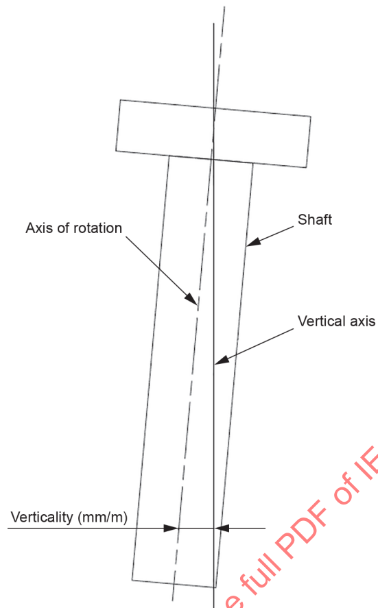
Figure 16 – Shaft verticality
