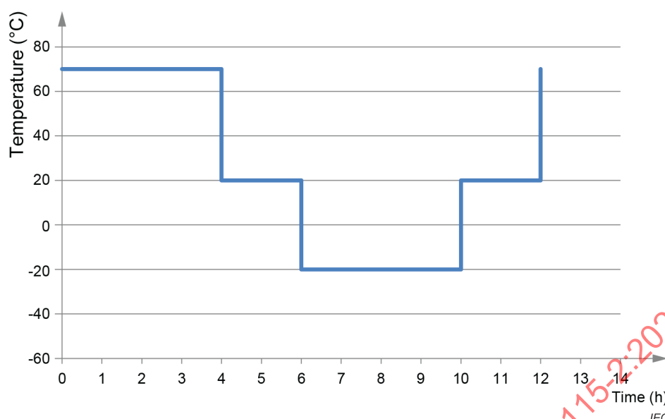
Figure 1 – Temperature profile for 6.4.3 – Temperature cycling test
