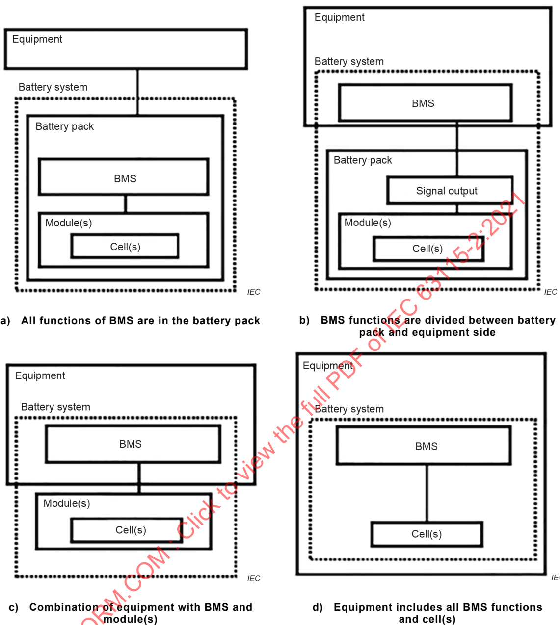
Figure 2 – Examples of BMS locations and battery system configurations
