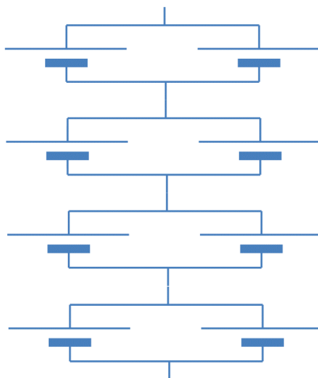
Figure A.4 – Structure 2P4S
