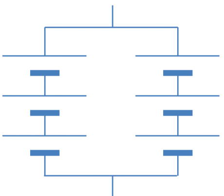
Figure A.3 – Structure 3S2P
