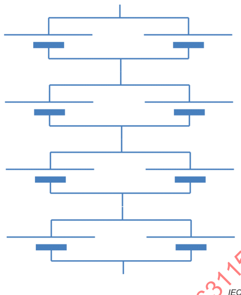
Figure A.4 – Structure 2P4S
