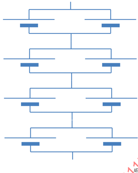
Figure A.4 – Structure 2P4S
