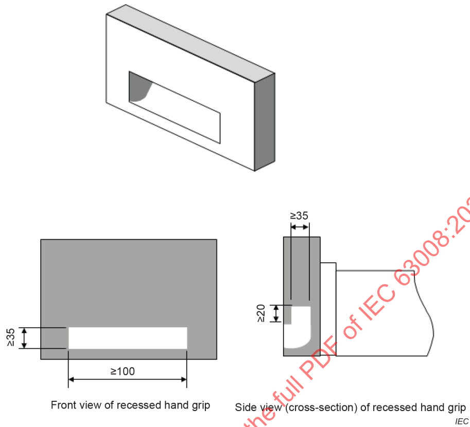
Figure 4 – Hand grip
