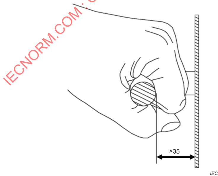
Figure 5 – Knuckle clearance when holding a handgrip
