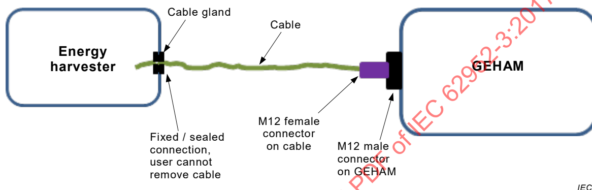
Figure A.1 – Option 1: Fixed connection on energy harvester, connector on GEHAM
