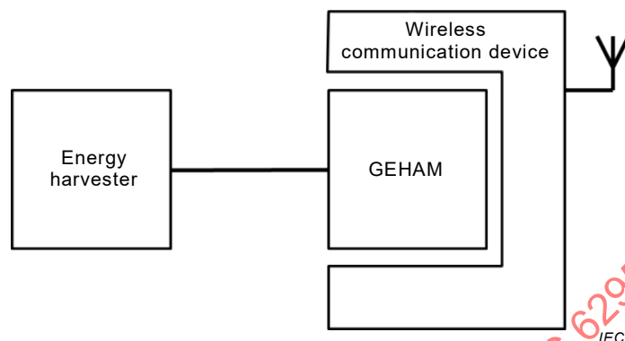
Figure A.6 – GEHAM is inside, energy harvester is outside of WCD
