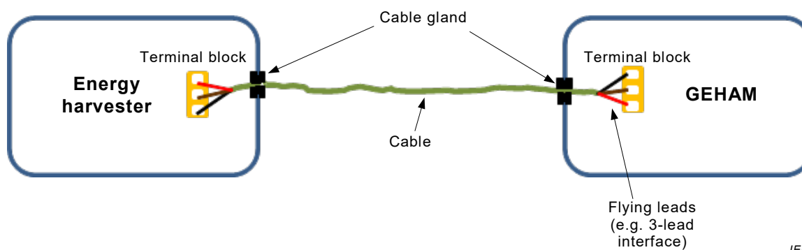
Figure A.5 – Option 5: Flying-lead interface on energy harvester, flying-lead interface on GEHAM side
