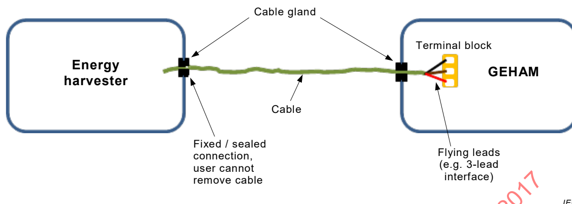
Figure A.3 – Option 3: Cable fixed on energy harvester, Flying Lead to GEHAM
