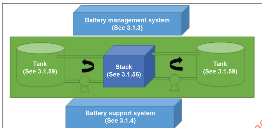
Figure 1 – Flow battery system (FBS)
