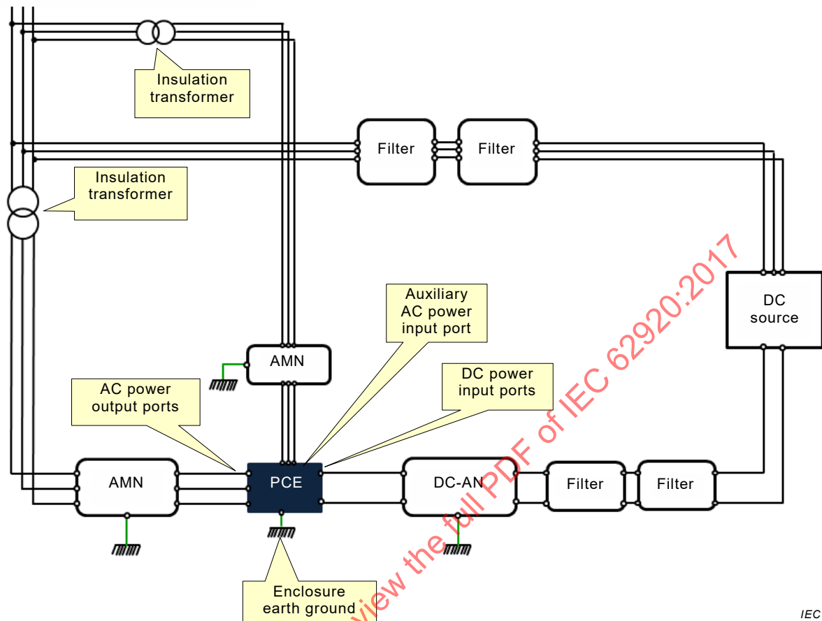
Figure C.2 – Example of a standardized test setup for conducted disturbances measurement with a laboratory AC power source
