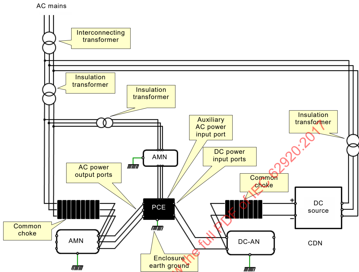
Figure D.4 – Alternative test method of conducted disturbances measurement using artificial networks as voltage probes
