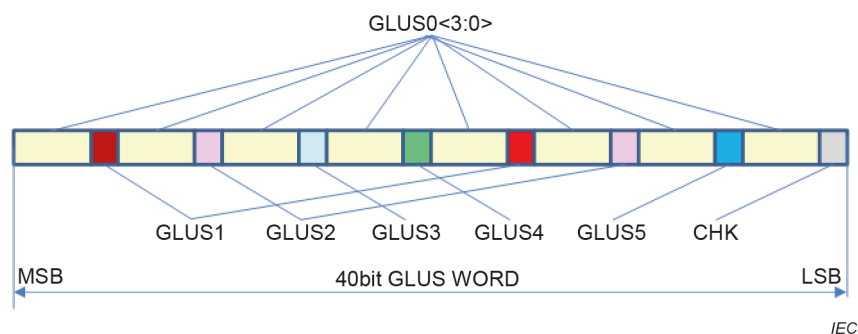
Figure 14 – Structure du mot GLUS
