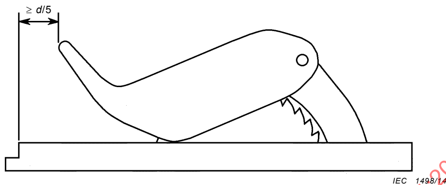
Figure 114 – Minimum distance from the front edge of the table top to the front edge of the saw blade guard
