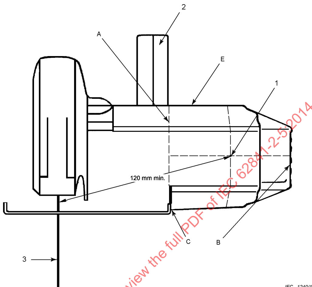
Figure 107b) – Circular saw without auxiliary handle (motor casing as grasping area)
