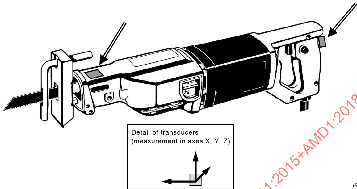
Figure I.103 – Positions of transducers for sabre saws
