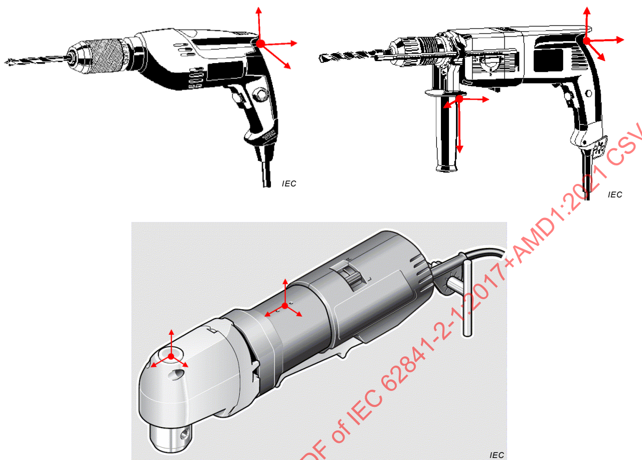
Figure I.102 – Positions of transducers for drills and impact drills
