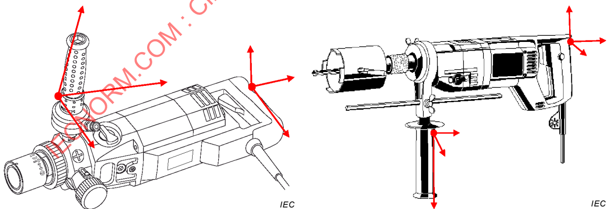
Figure I.103 – Positions of transducers for diamond core drills
