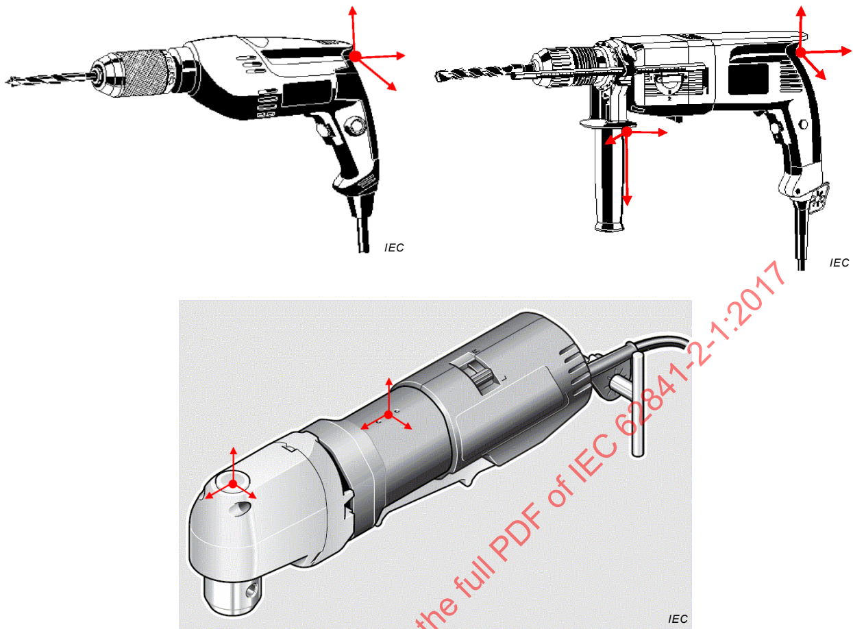
Figure I.102 – Positions of transducers for drills and impact drills
