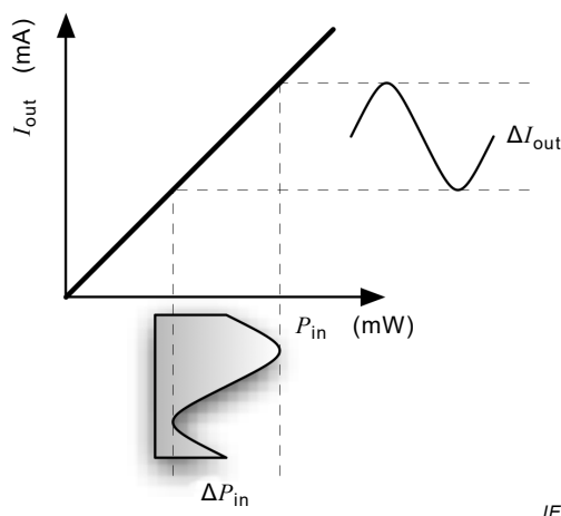
Figure 1 – Definition of "conversion efficiency "
