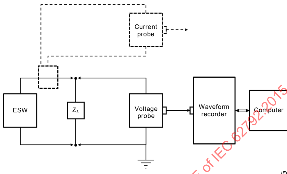
Figure 1 – Diagram of the ESW measurement system with voltage and current probes in place
