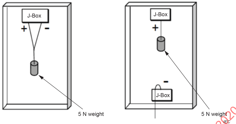
a) Utilizing the leads
