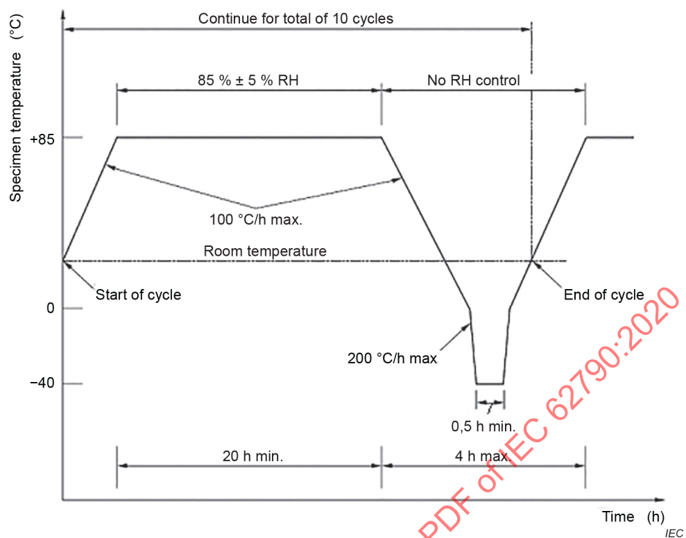
Figure 2 – Humidity-freeze cycle
