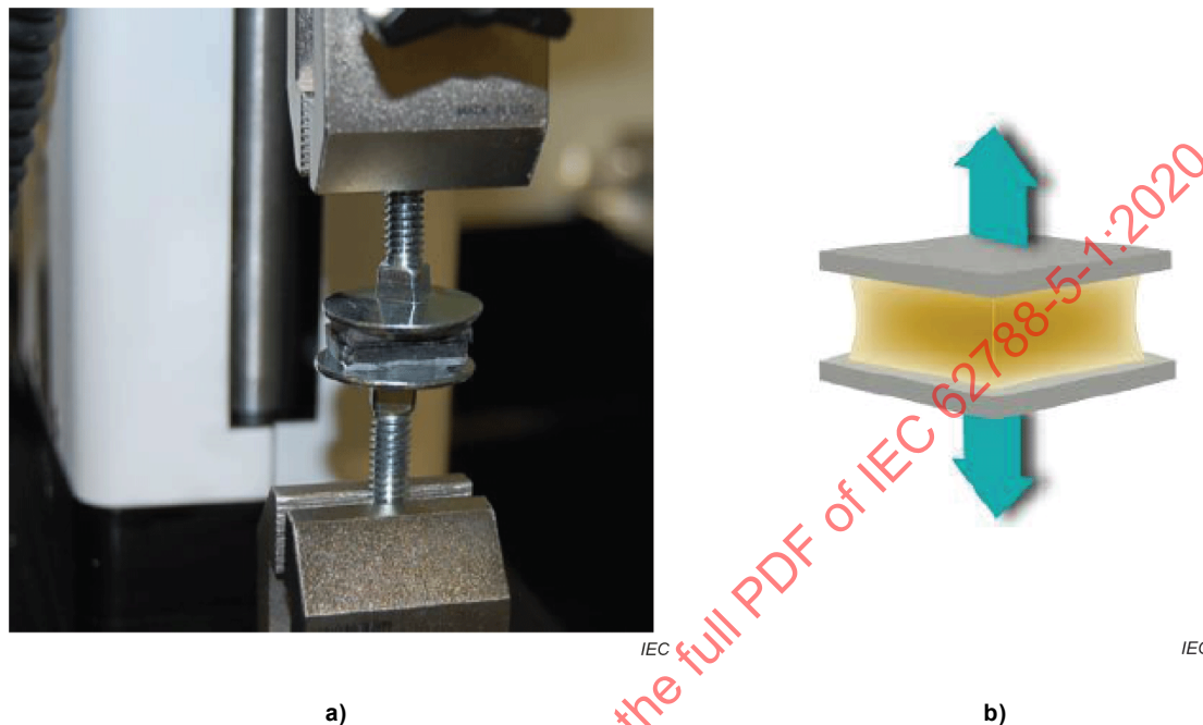
Figure 2 –Photograph (a)) and schematic (b)) of a z-tensile adhesion test specimen
