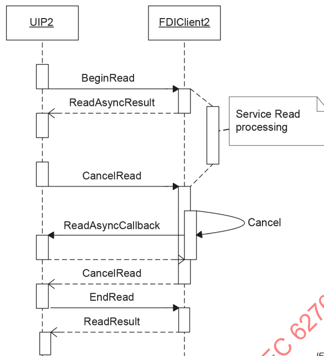
Figure 7 – Cancel service processing sequence example
