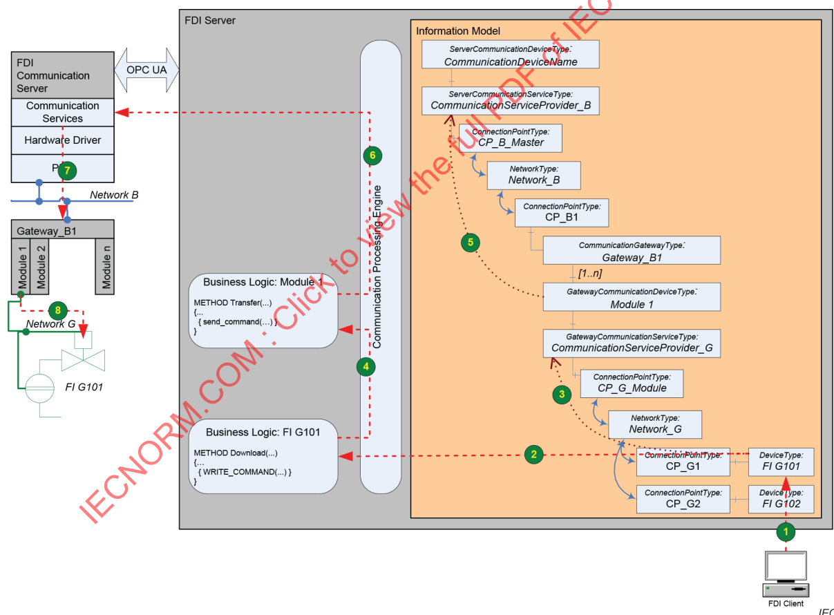
Figure 23 – Message propagation example scenario
