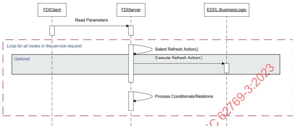
Figure 7 – Offline variable read
