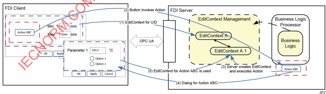
Figure 6 – EditContext for EDD Methods
