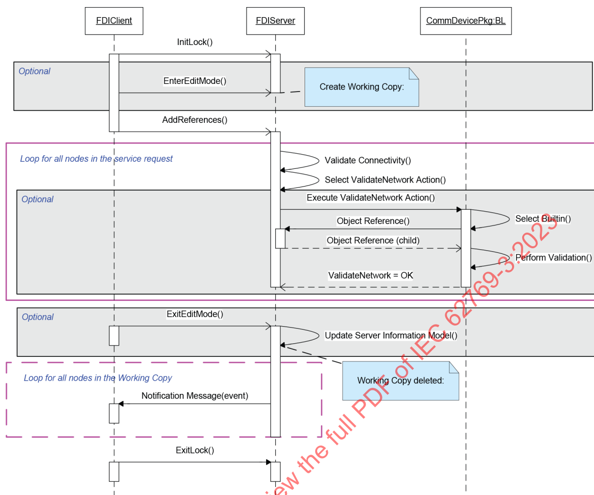
Figure 15 – Add Device to topology
