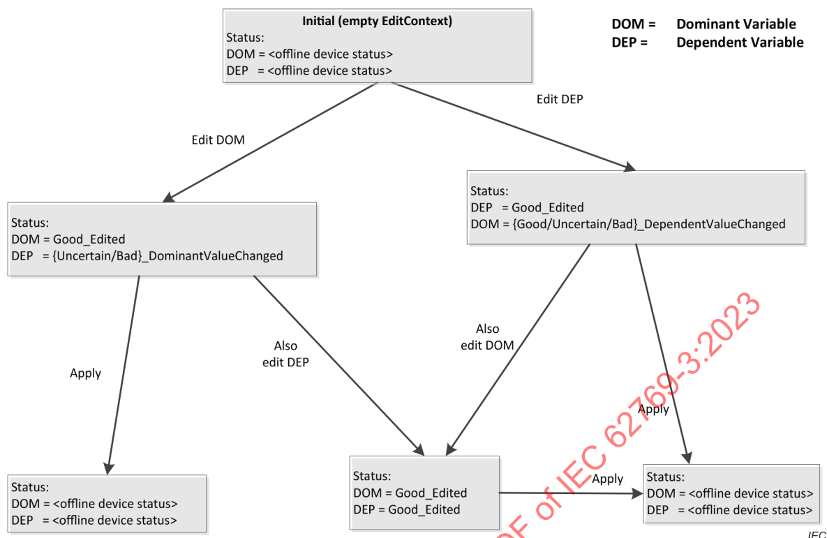
Figure 5 – Offline EditContext state diagram for dominant and dependent Variables
