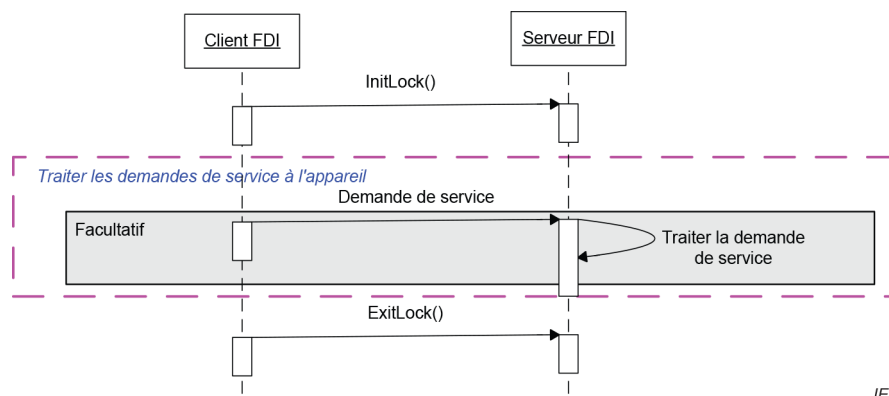
Figure 2 – Services de verrouillage
