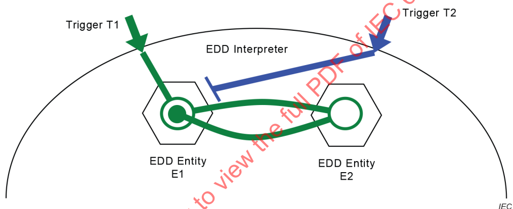
Figure C.4 – Concurrent execution of two triggers (step 3)
