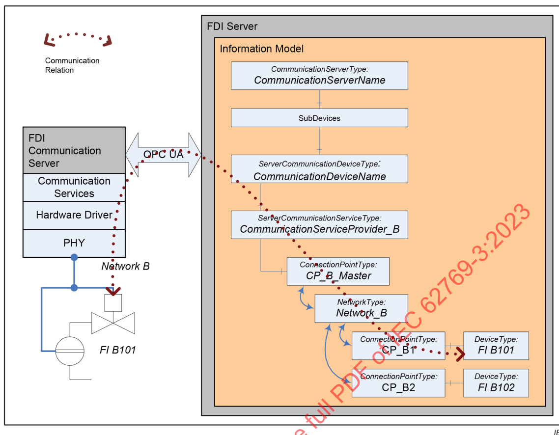
Figure 21 – FDI® Communication Server integration example
