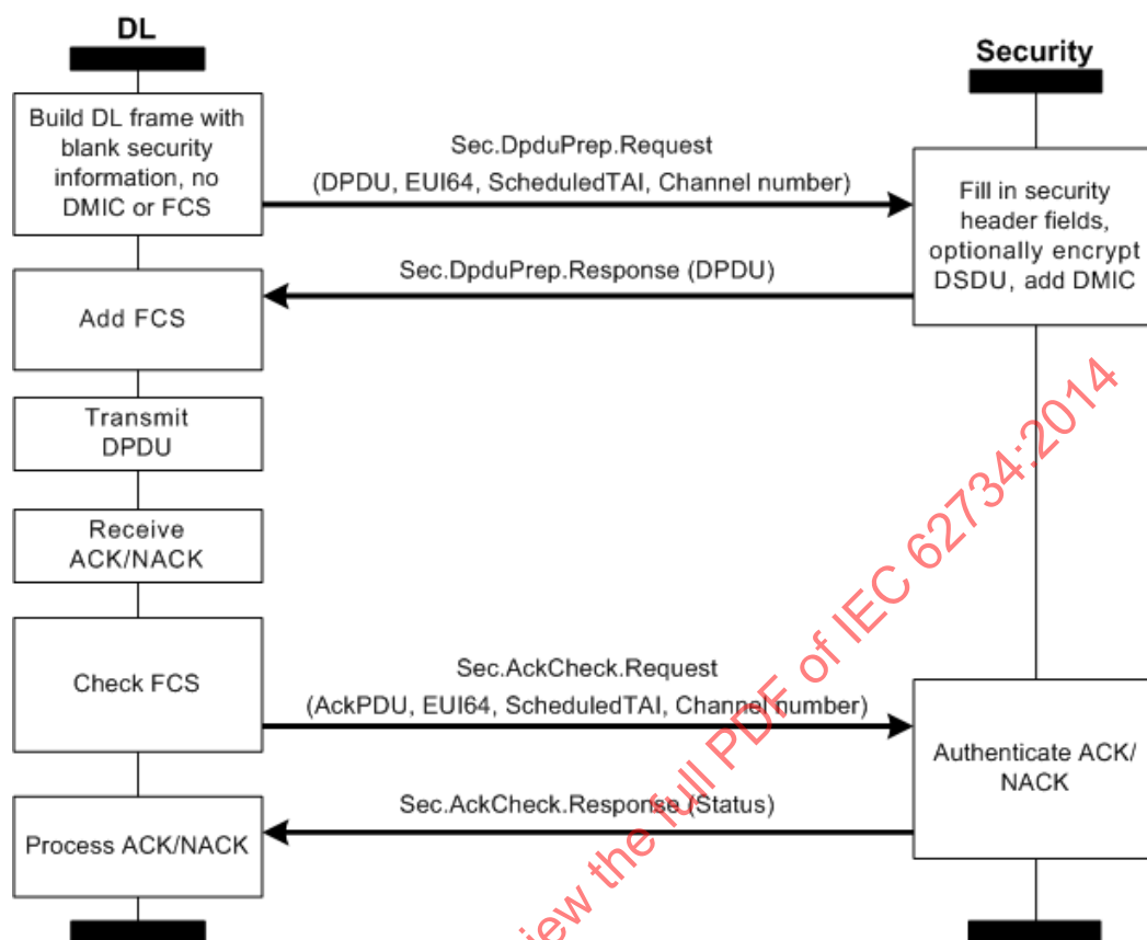
Figure 38 – DLE and DSC processing for a D-transaction initiator
