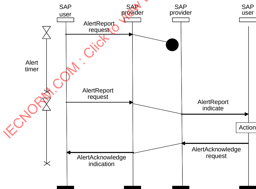
Figure 131 – AlertReport, delivery failure
