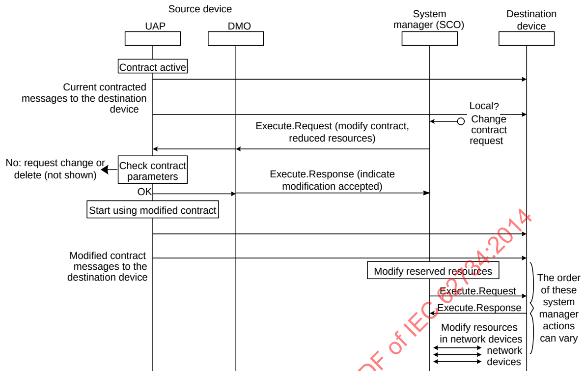
Figure 33 – Contract modification with immediate effect
