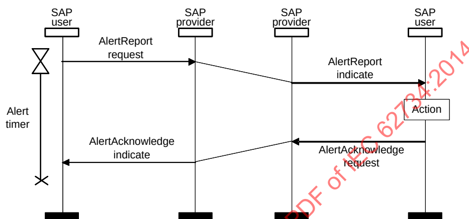
Figure 130 – AlertReport and AlertAcknowledge, delivery success
