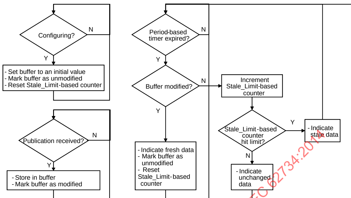
Figure U.22 – Publish/subscribe subscriber common periodic and CoSt flowchart
