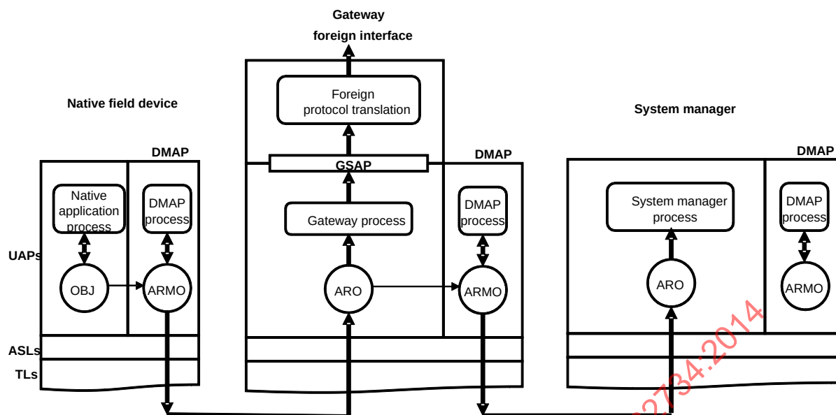
Figure U.29 – Alert cascading
