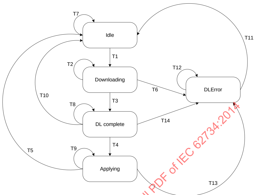
Figure 123 – UploadDownload object download state diagram
