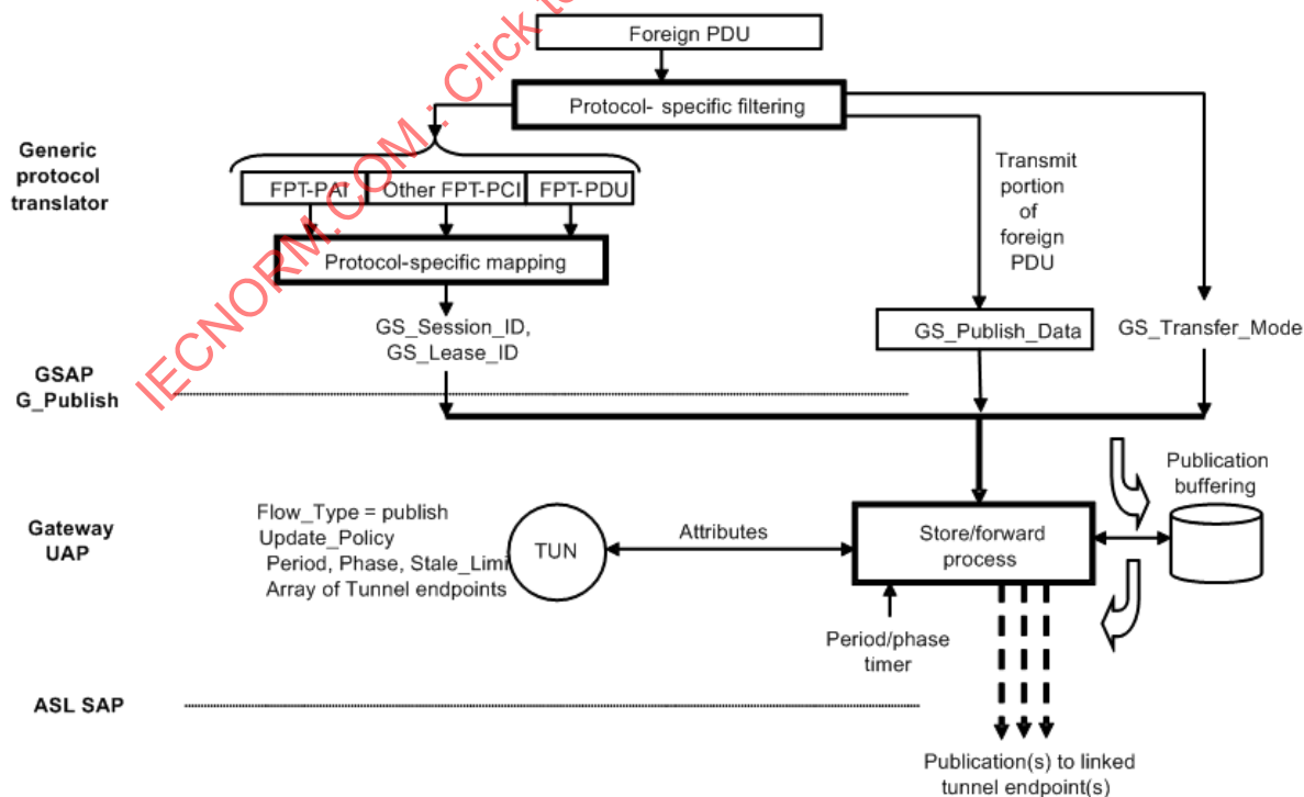
Figure O.1 – Generic protocol translation publish diagram
