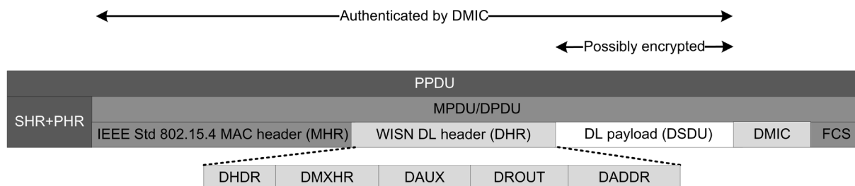
Figure 37 – DPDU structure
