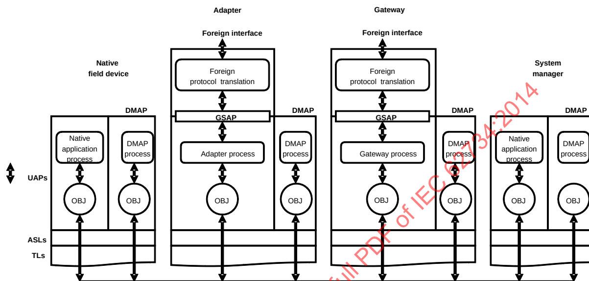
Figure U.2 – Basic gateway model
