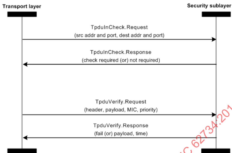
Figure 43 – TL and TSC interaction, incoming TPDU
