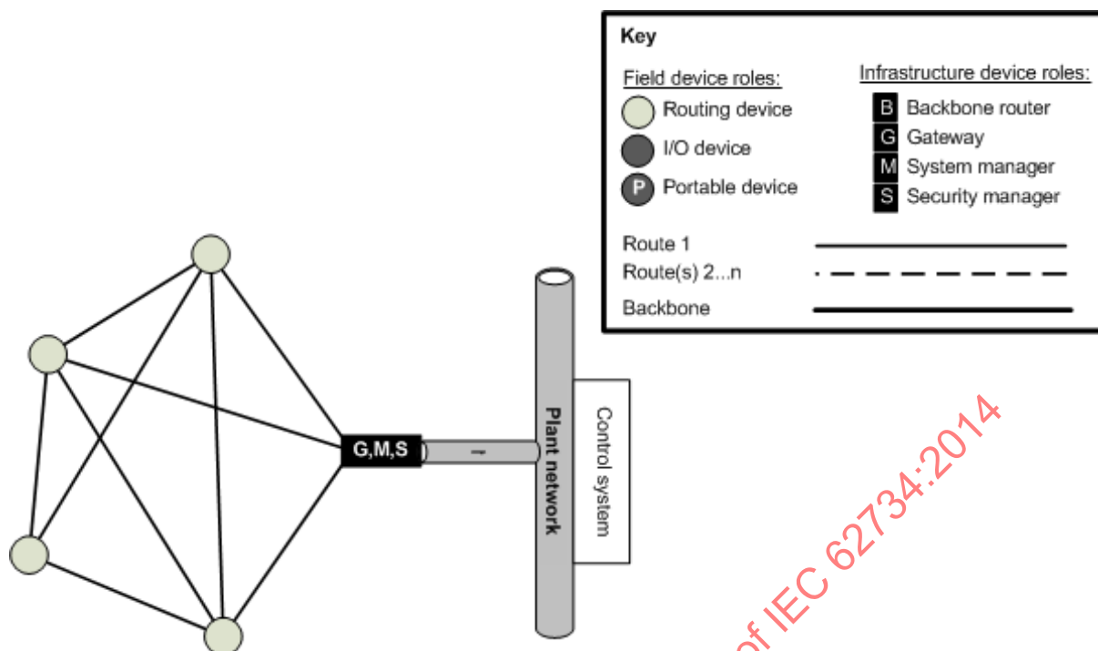
Figure 8 – Mesh topology
