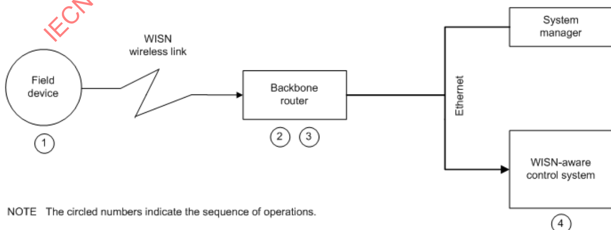
Figure 104 – Example of routing over an Ethernet backbone network
