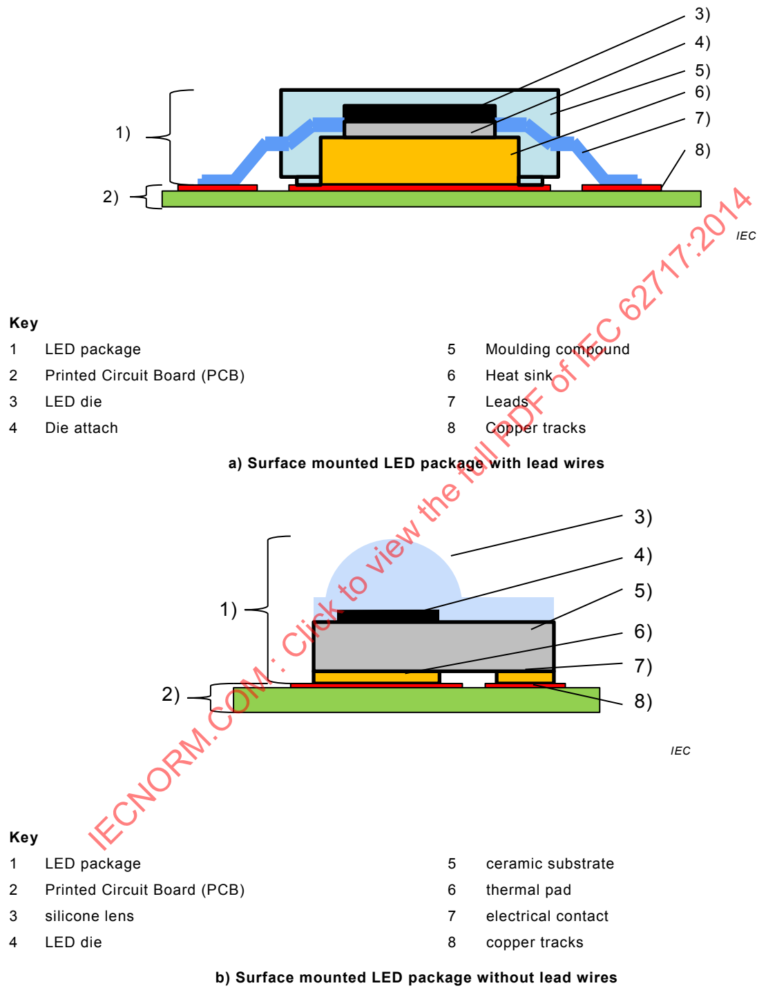
Figure G.2 – Schematic drawings of LED packages
