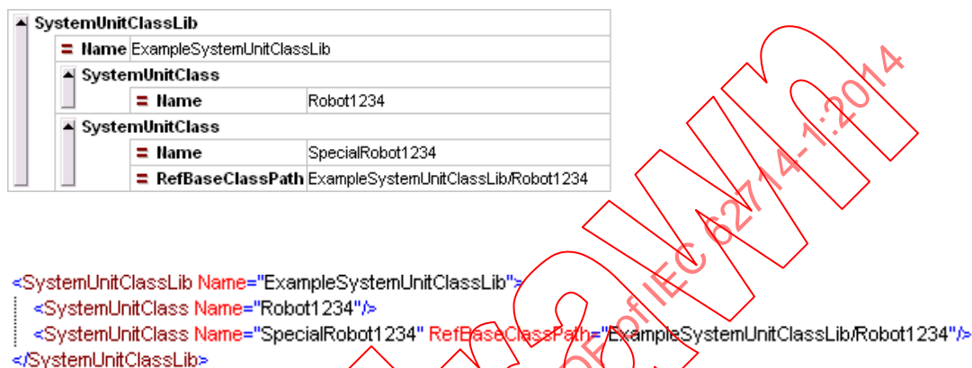
Figure 4 – Object identification example of an AML class
