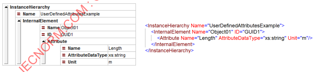
Figure 14 – Example of a user-defined attribute
