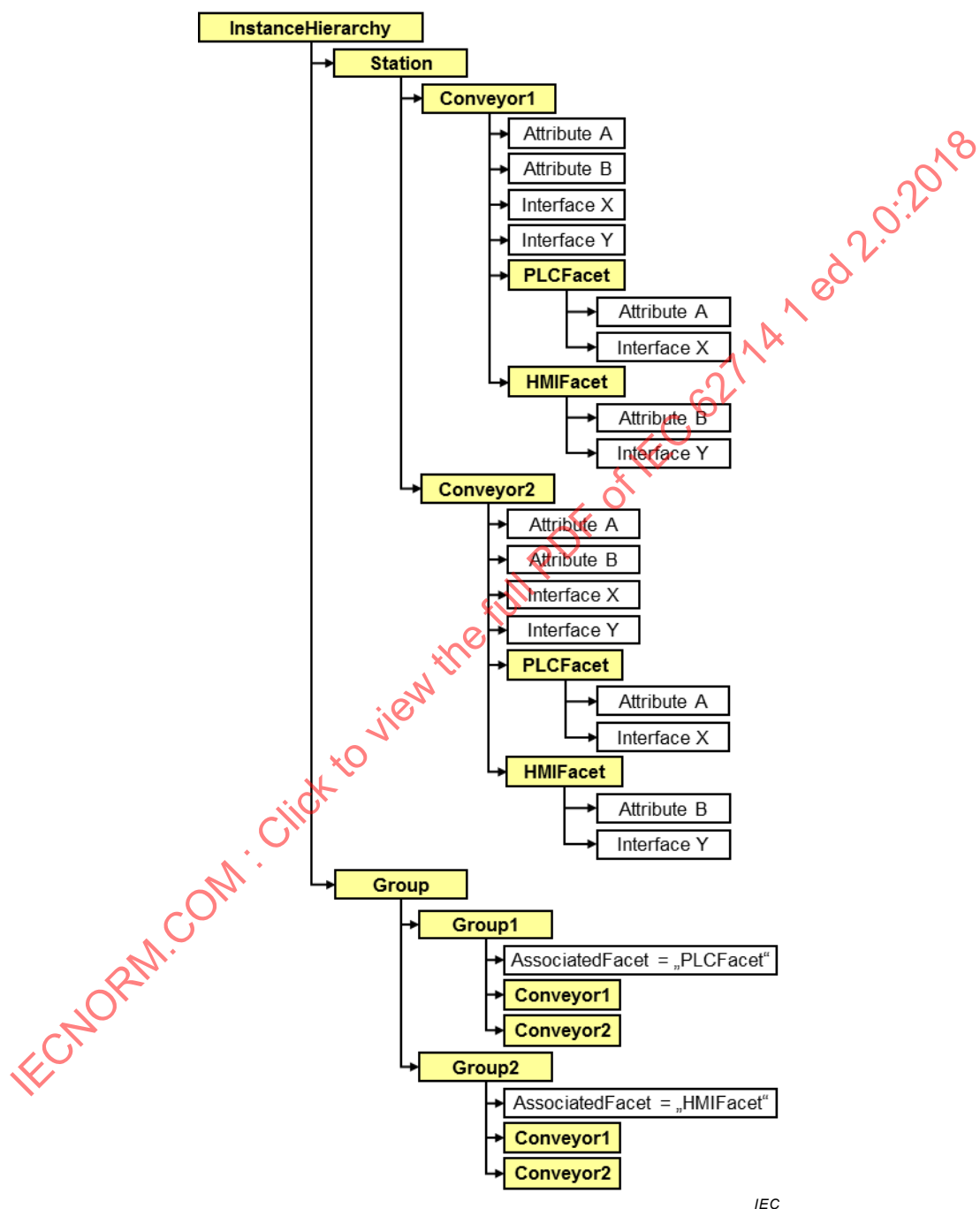
Figure A.22 – Combination of the Facet and Group concept
