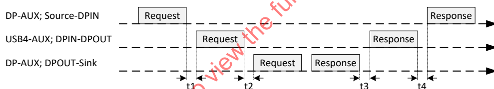
Figure 10-15. AUX Timing
