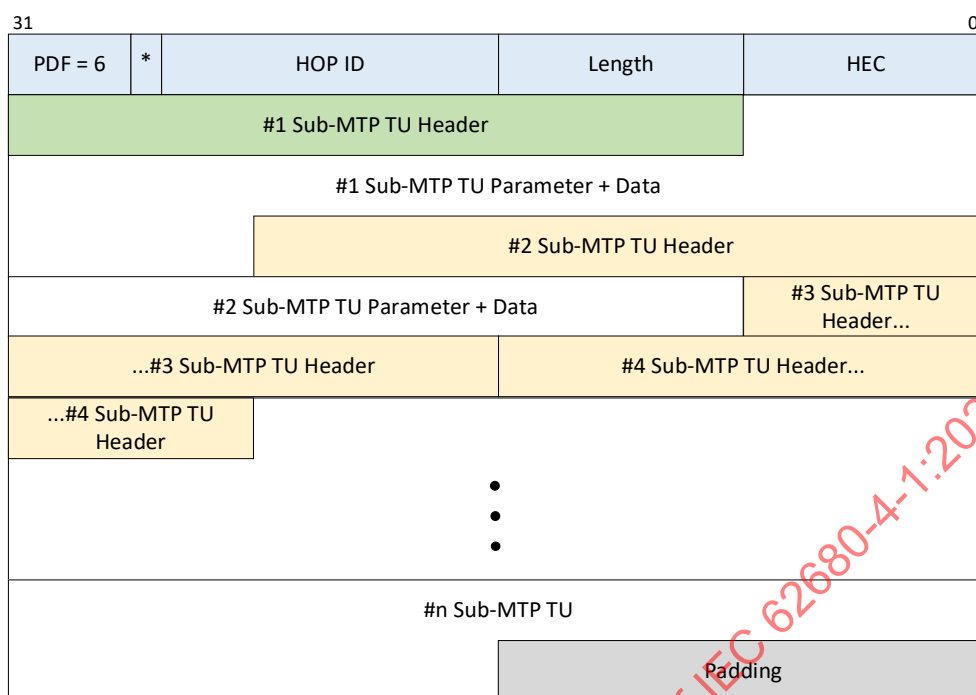
Figure 10-46. MST Packet Format
