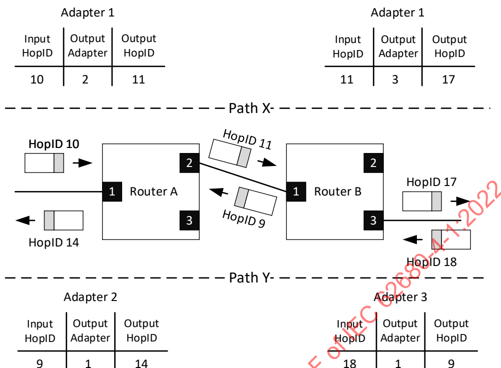
Figure 5-9. Routing Example
