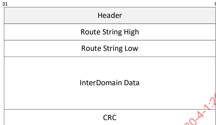
Figure 6-14. Inter-Domain Response
