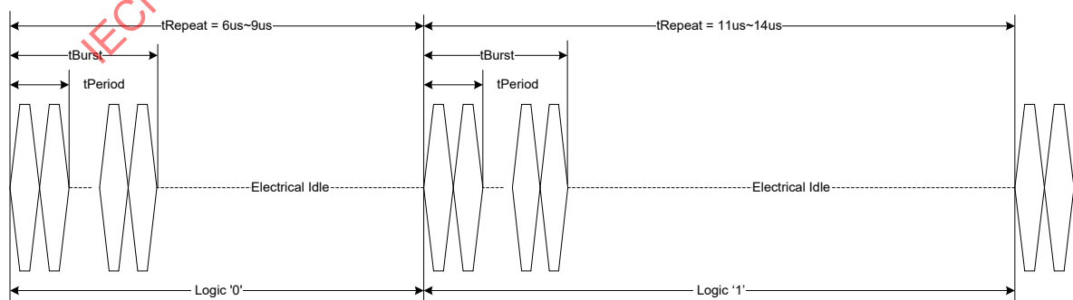
Figure 6-32 – Example of Binary Representation based on Polling.LFPS
