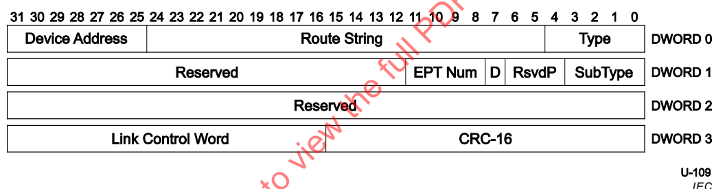
Figure 8-28 – PING Transaction Packet
