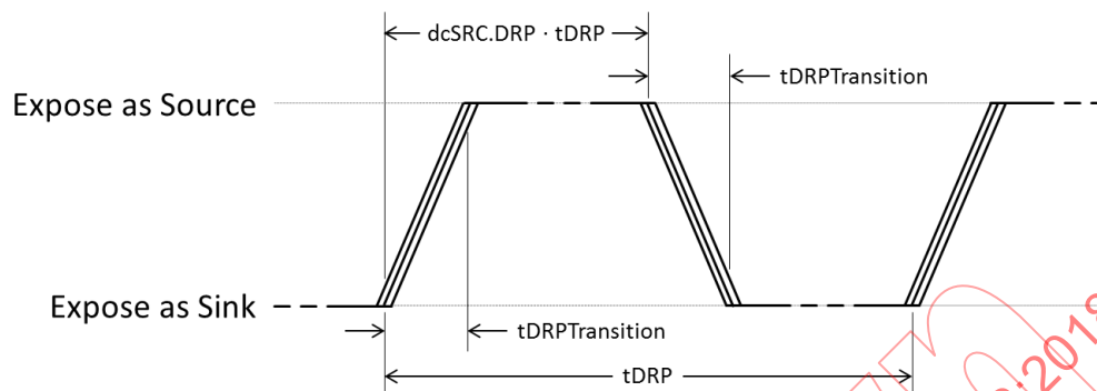
Figure 4-42 DRP Timing
