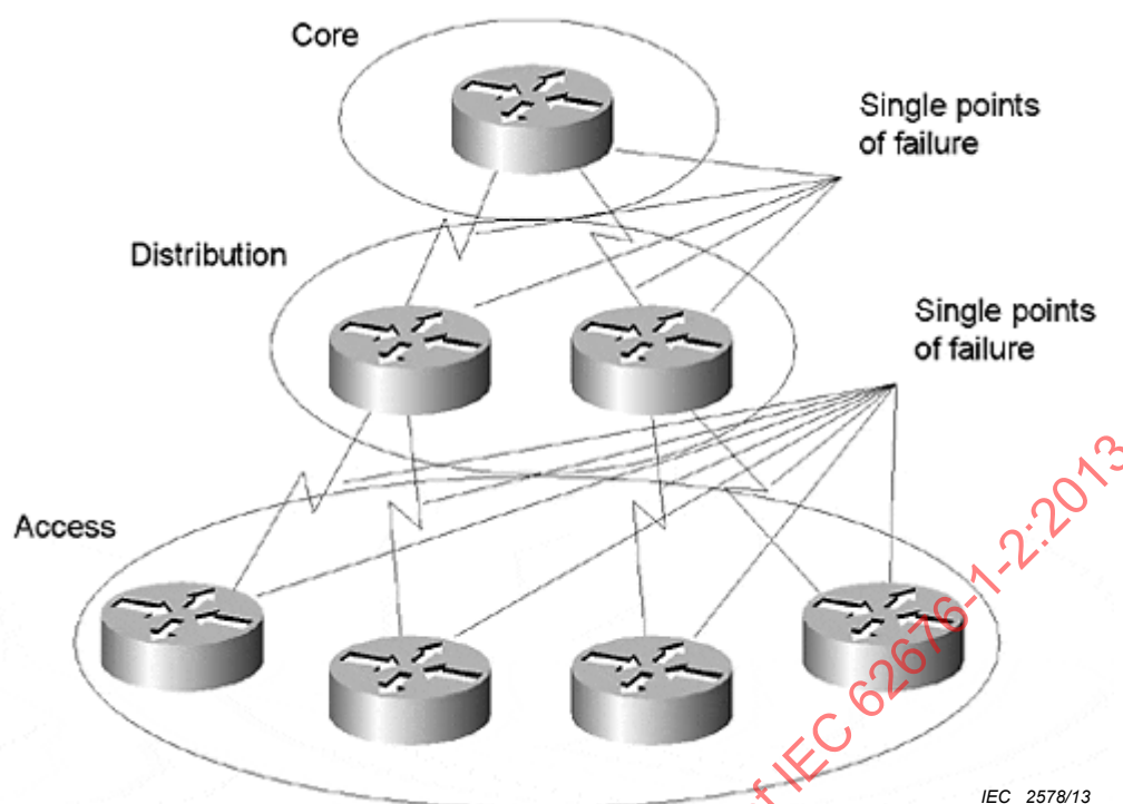
Figure 6 – Hierarchical network
