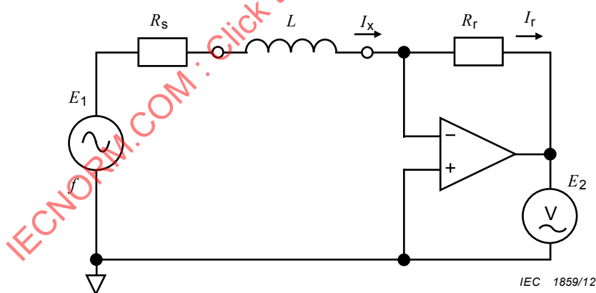
Figure 4 – Example of a circuit for measurement by the automatic balancing bridge method
