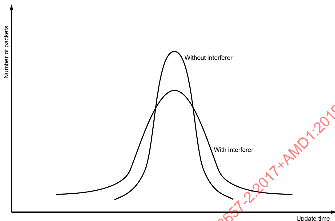
Figure 21 – Example of distribution functions of the update time
