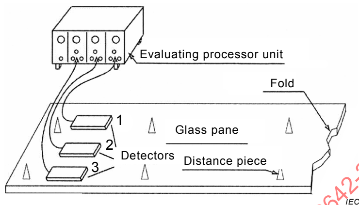
Figure K.1 – Passive surface mounted glass break detectors test setup
