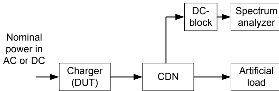
Figure 4 – Test set up for high frequency voltage components
