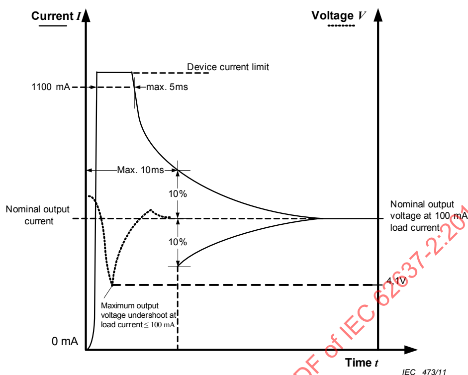
Figure 1 – Maximum duration of charging current overshoot and output voltage undershoot
