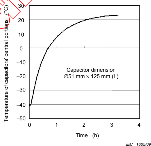
Figure B.4 – Temperature changes of capacitors' central portions ( -40\text{ }^{\circ}\text{C} \rightarrow 25\text{ }^{\circ}\text{C} )
