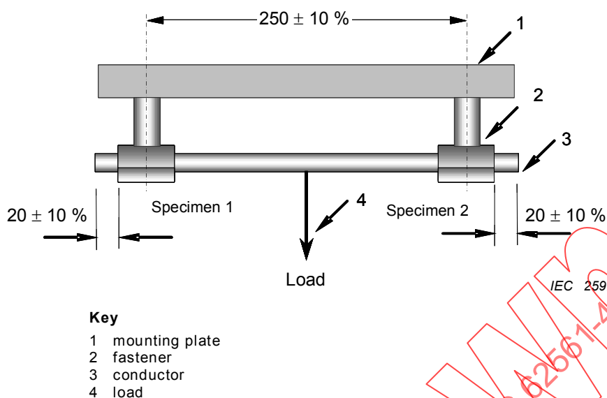
Figure 2 – Basic arrangement of lateral load test
