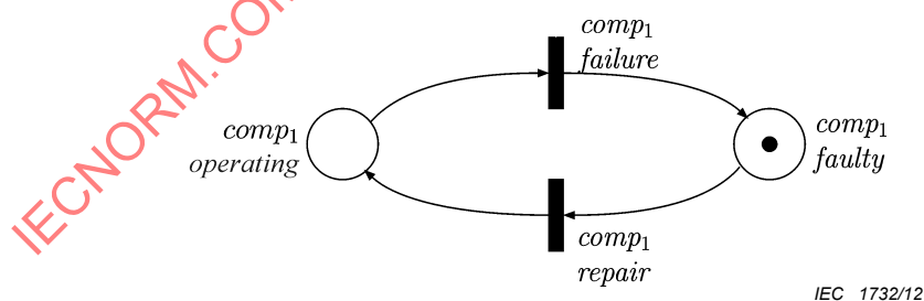
Figure A.1 – Availability state-transition circle of a component
