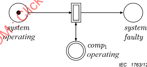
Figure C.3 – Basic reliability and function modelling concept
