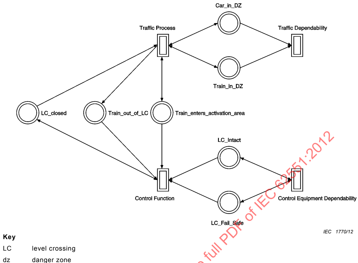
Figure E.3 – Submodels of the level crossing example model
