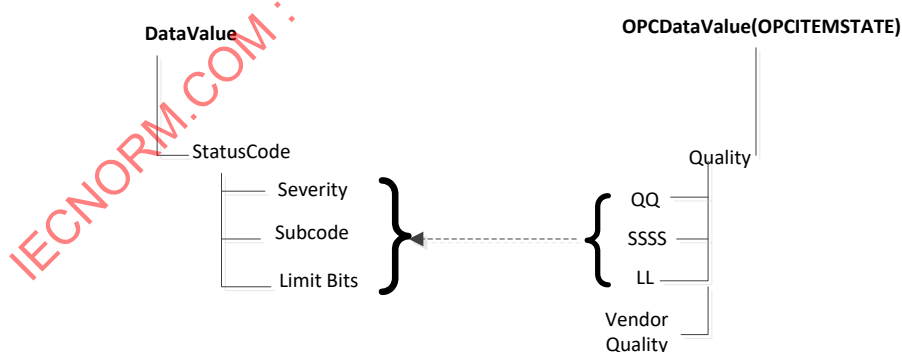
Figure A.3 – Status Code mapping
