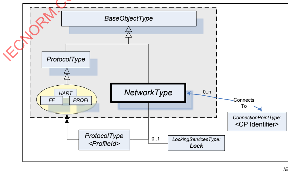
Figure 15 – NetworkType
