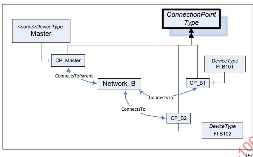
Figure 18 – ConnectionPoint usage
