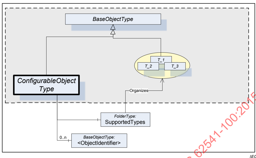
Figure 13 – ConfigurableObjectType
