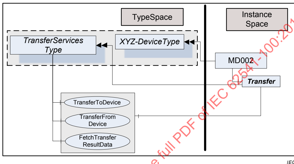
Figure 26 – TransferServices
