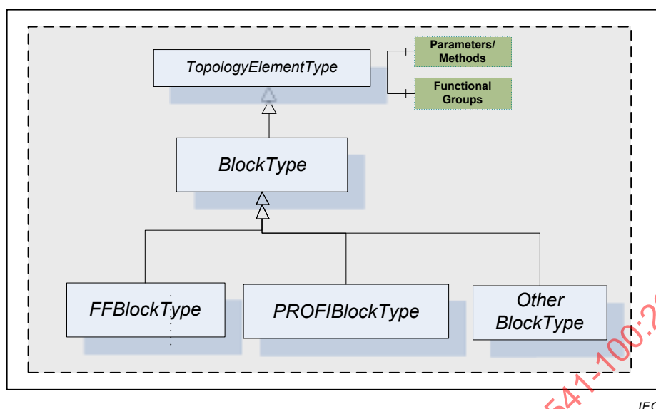
Figure 11 – BlockType hierarchy
