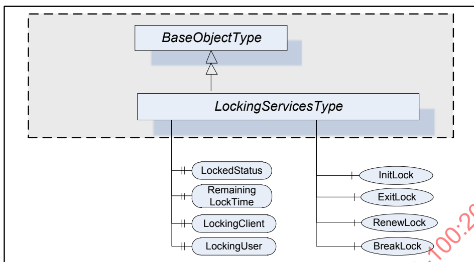
Figure 27 – LockingServicesType
