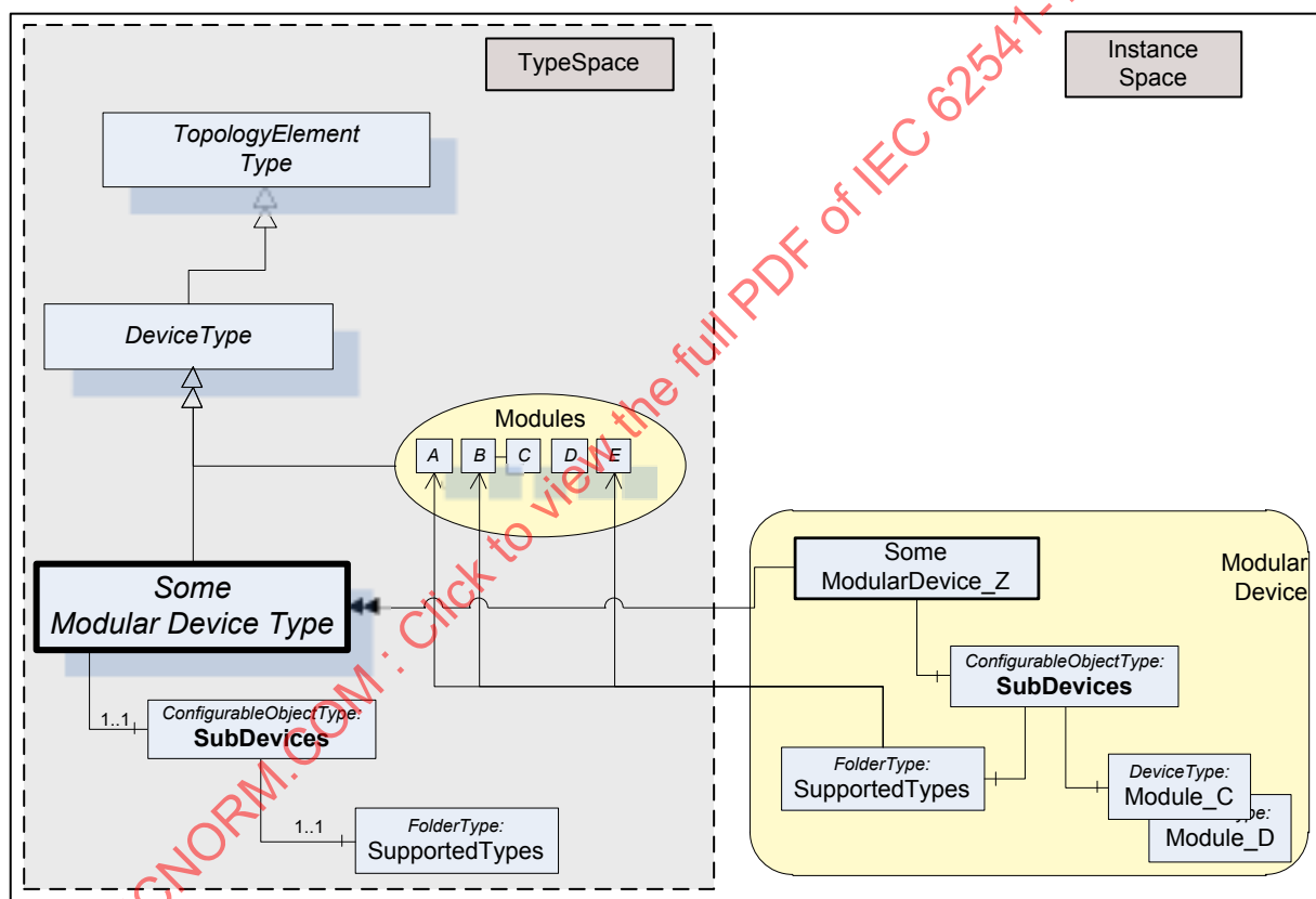
Figure 30 – Modular Device structure example
