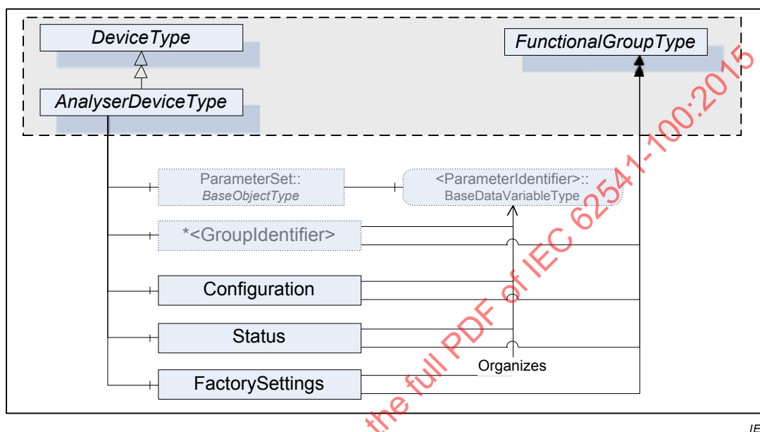
Figure 4 – AnalysersDeviceType use for FunctionalGroups (UA Companion ADI)
