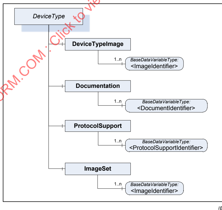
Figure 8 – Integration of support information within a DeviceType
