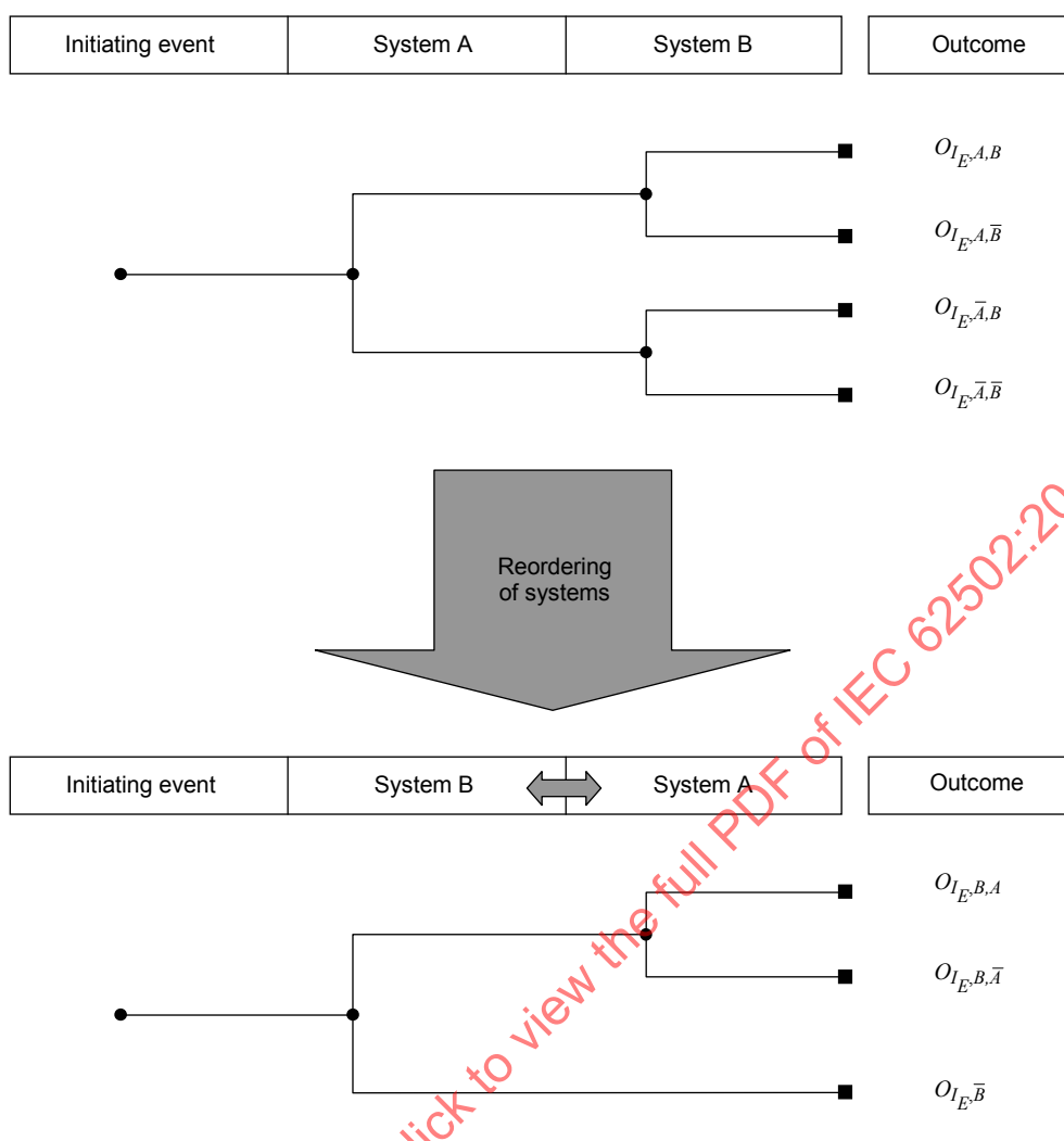
Figure 3 – Functional dependencies in event trees
