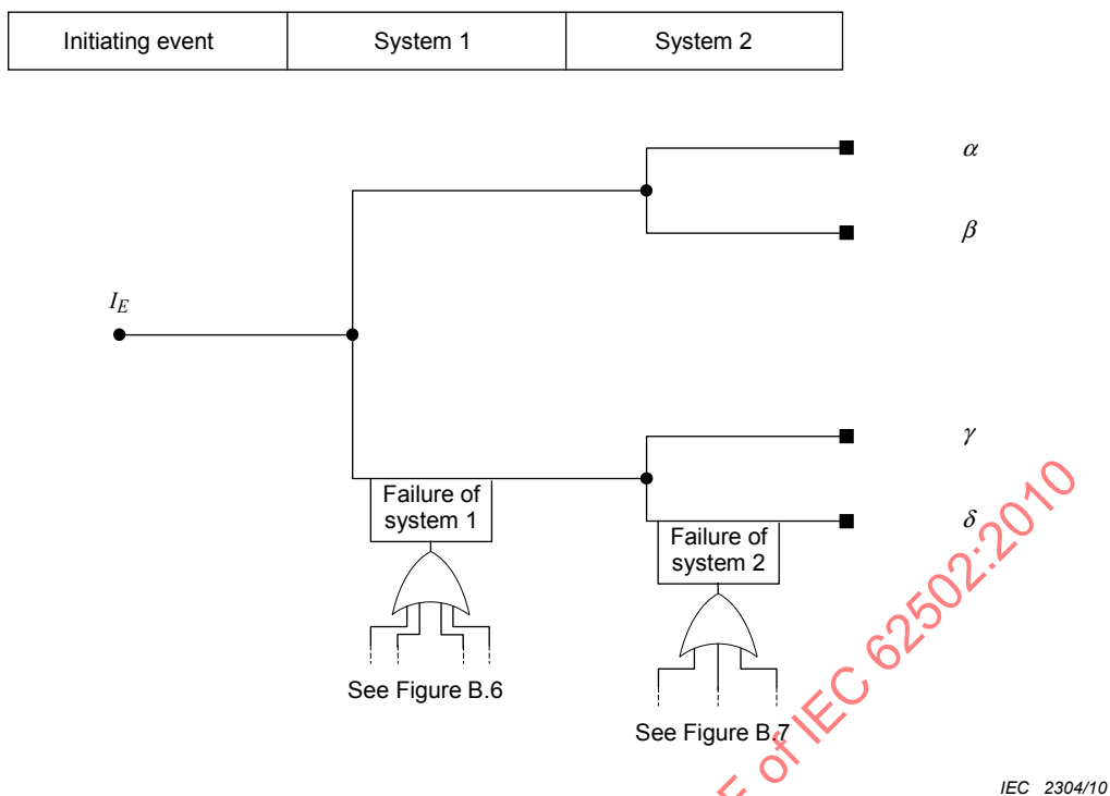
Figure B.5 – Simple example
